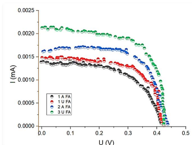
2-rasm. Fotoanod uchun ananaviy va ultratovushli tasir asosida tayyorlangan namunalarning JV tavsifi
