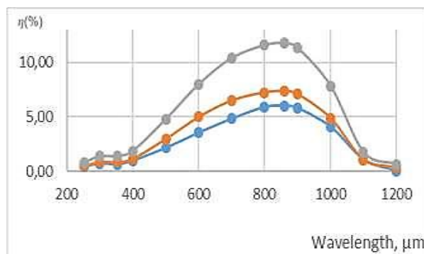
Fig. 2. Spectral sensitivity and dependence of the maximum voltage of a polycrystalline silicon photocell at various light intensities
