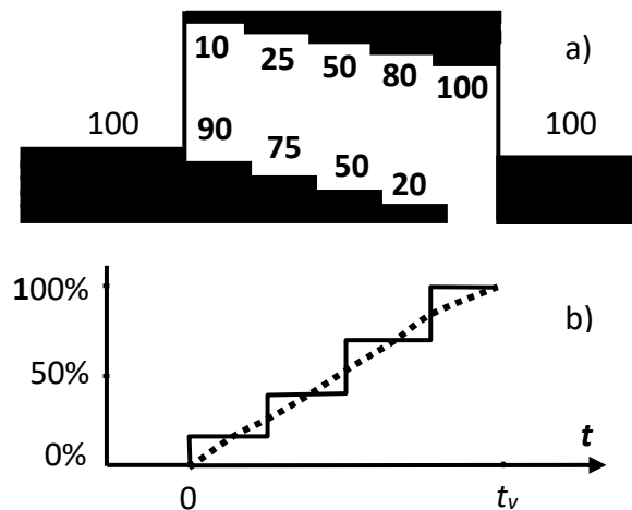
Fig. 1. a) - schematic distribution of the optical blackening density on the oscillogram of the current pulse, b) - time dependence of the average current obtained from oscillogram (a).
