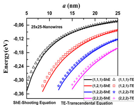
2-rasm. InP/InAs 0.25 P 0.75 /InP geterotuzilmasining 25×25 o'lchamli InAs 0.25 P 0.75 nanosimi ichidagi kubik shakldagi InAs kvant nuqtaning o'lchamiga bog'liq holda yengil kovaklarning energiya satxlari o'zgarishi.
