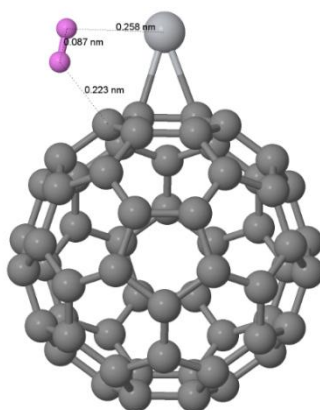
Figure 2. Optimized structure of stable M@C 60 complexes (M=Ti) with M–C bond distances mentioned at the calculated using the LAMMPS package.
