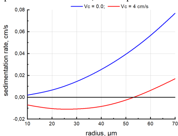
Figure 2. Dependence of the sedimentation rate on the radius R of a particle
