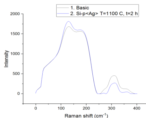
Figure 3b. Magnified view of the spectral region up to 400 \text{ cm}^{-1} .
