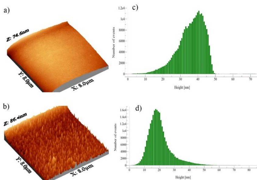
Figure 1. AFM surface morphology (a, b) and corresponding height distribution histograms (c, d) of \text{Ga}_2\text{O}_3 thin films annealed at 1000 °C (a, c) and 1100 °C (b, d) for 2 hours.
