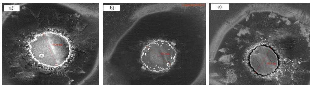
2-rasm. Lazer energiya oqimlari a) 16.37 \text{ J/cm}^2 , b) 17.81 \text{ J/cm}^2 , c) 21.17 \text{ J/cm}^2 natijasida Alyuminiy folga ustidagi ablyatsion kraterlarining SEM mikroskop yordamida olingan tasvirlari
