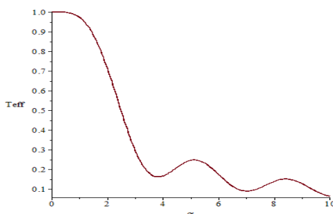
1-rasm. Tunnellanish koeffitsienting modulyatsiya parametriga bog'liqligi.
