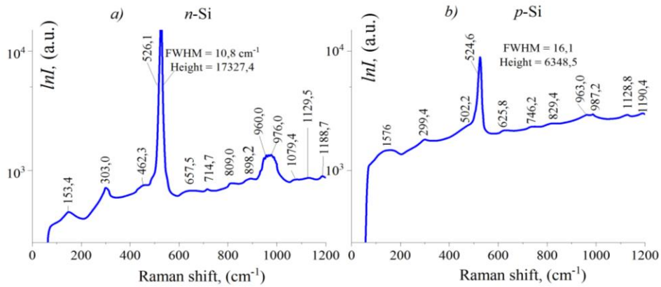
Figure 1. Raman spectra of n-Si and p-Si samples
