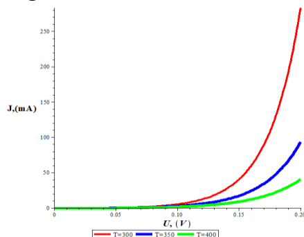
1-rasm. Dember effektining harorat ta'sirida VAX o'zgarishi
