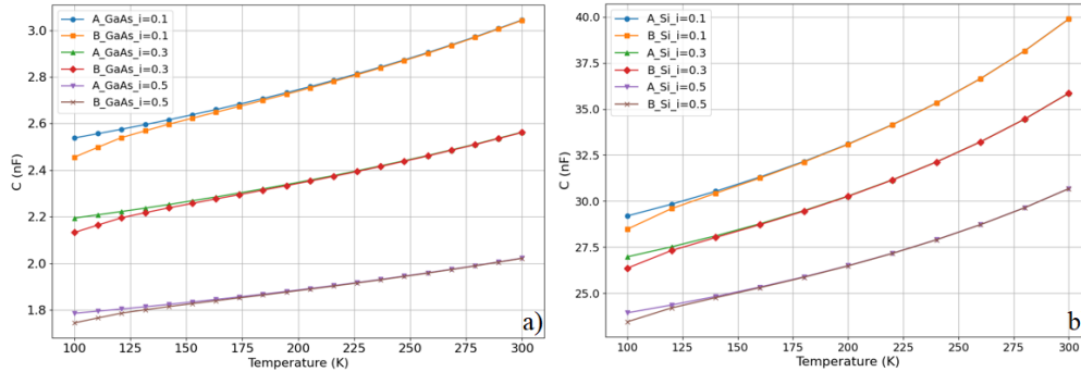
Figure 1. C–V characteristics of radial p–n junction structures: a) GaAs, b) Si
