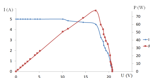
2-рasm. Mexanik kuchlanish ostida bo‘lgan quyosh panelining VAXi
