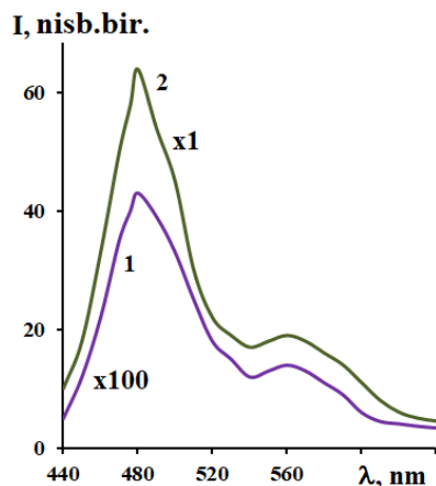
1-rasm. Oddiy (silindrsimon) kyuveta (1) va rezonatorli kyuveta (2) dagi ZnSe mikrokukunlarining ( d_{\text{ort}}=2 \text{ mkm} ) FL spektrlari ( I_{\text{uyg}} \sim 10^5 \text{ Vt/sm}^2 ).
