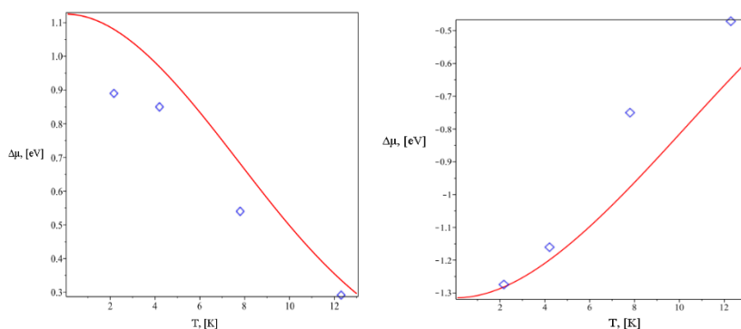
1-rasm. Kimyoviy potensial o'zgarishining haroratga bog'lanishi.
