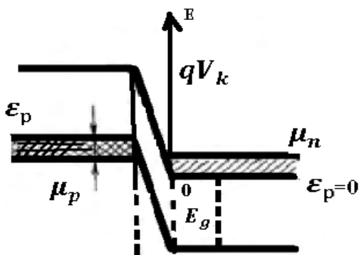
1-rasm. Tunnel o'tishning zonalar bo'yicha sxematik ko'rinishi
