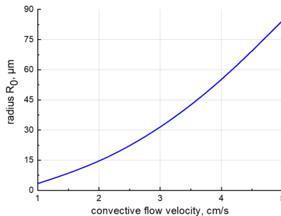
Figure 1. Dependence of the radius R_0 on the velocity of the convective air flow
