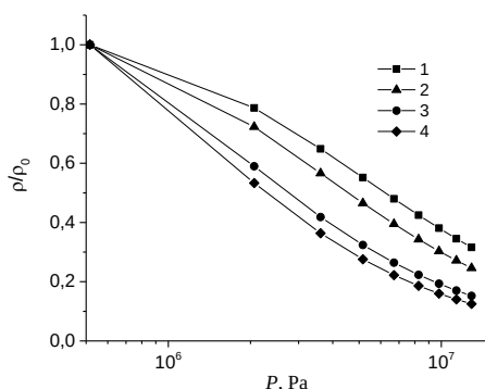
1-rasm. Turli haroratlarda bosim ta'sirida klasterlarga ega kremniy namunalarning ( \rho = 5.5 \cdot 10^3 \text{ Om} \cdot \text{sm} ) solishtirma qarshiligining nisbiy o'zgarishi: 1 – 30 °C, 2 – 40 °C, 3 – 50 °C, 4 – 70 °C.
