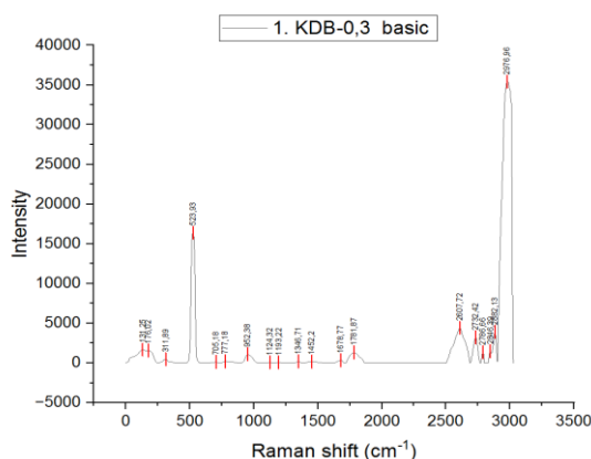
Fig/ 1. Raman spectrum of the initial sample with a conductivity of \sigma = 0.45 \text{ } \Omega^{-1} \cdot \text{cm}^{-1} .
