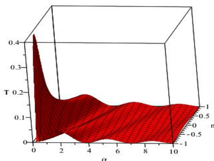
2-rasm: Shaffoflik koeffitsientining \alpha va n ga bog'liqligi
