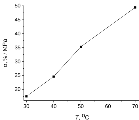
2-rasm. Namunalarning \alpha tenzosezgirlikining harorat ta'sirida o'zgarishi.
