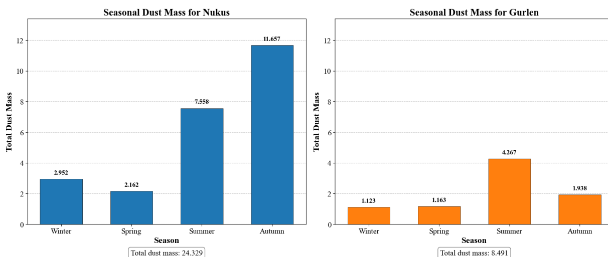
Fig.1. Comparison of seasonal dust mass
