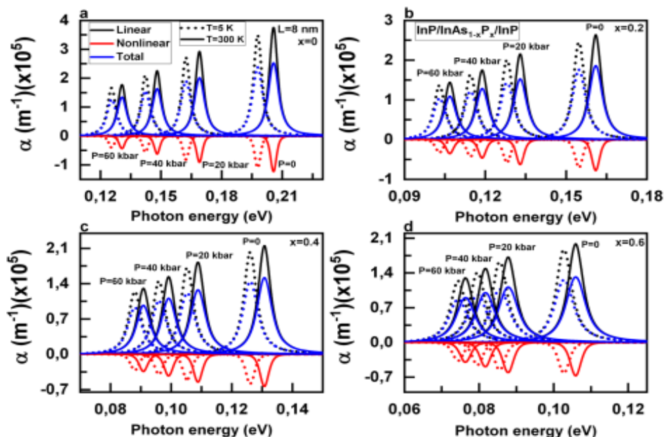
1-rasm. \text{InP}/\text{InAs}_{1-x}\text{P}_x/\text{InP} kvant o'rasi uchun yutilish koefitsientining foton energiyasiga bog'liqligi
