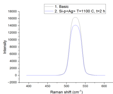
Figure 3c. Magnified view of the spectral region from 400 cm -1 to 600 cm -1 .
