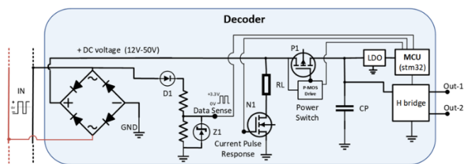
Figure 5: Decoder device
