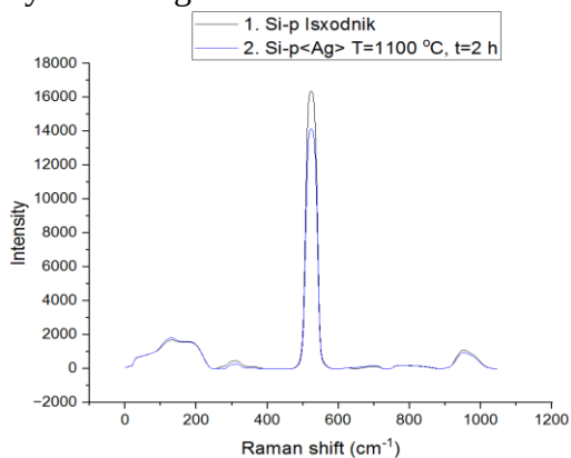
Figure 3a. Overlay of the overall Raman spectra of the initial and silver-diffused samples.
