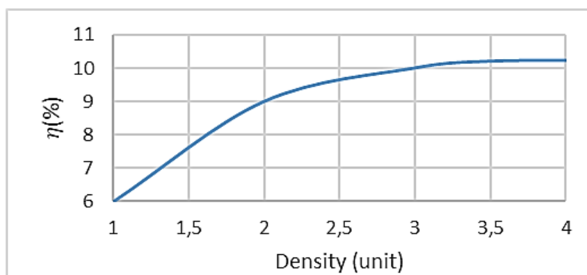
Fig. 3. The dependence of the efficiency transforming a solar cell from selective radiation density.
