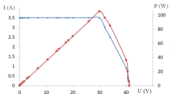
1-рasm. Mexanik kuchlanish ostida bo‘lmagan quyosh panelining VAXi
