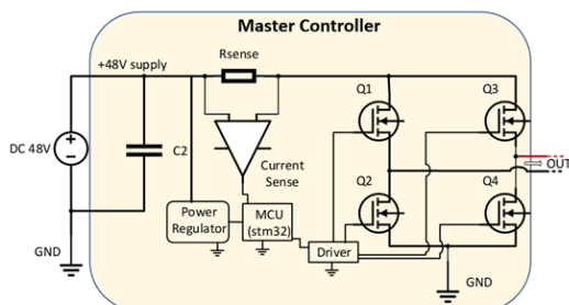
Figure 4: Master Controller
