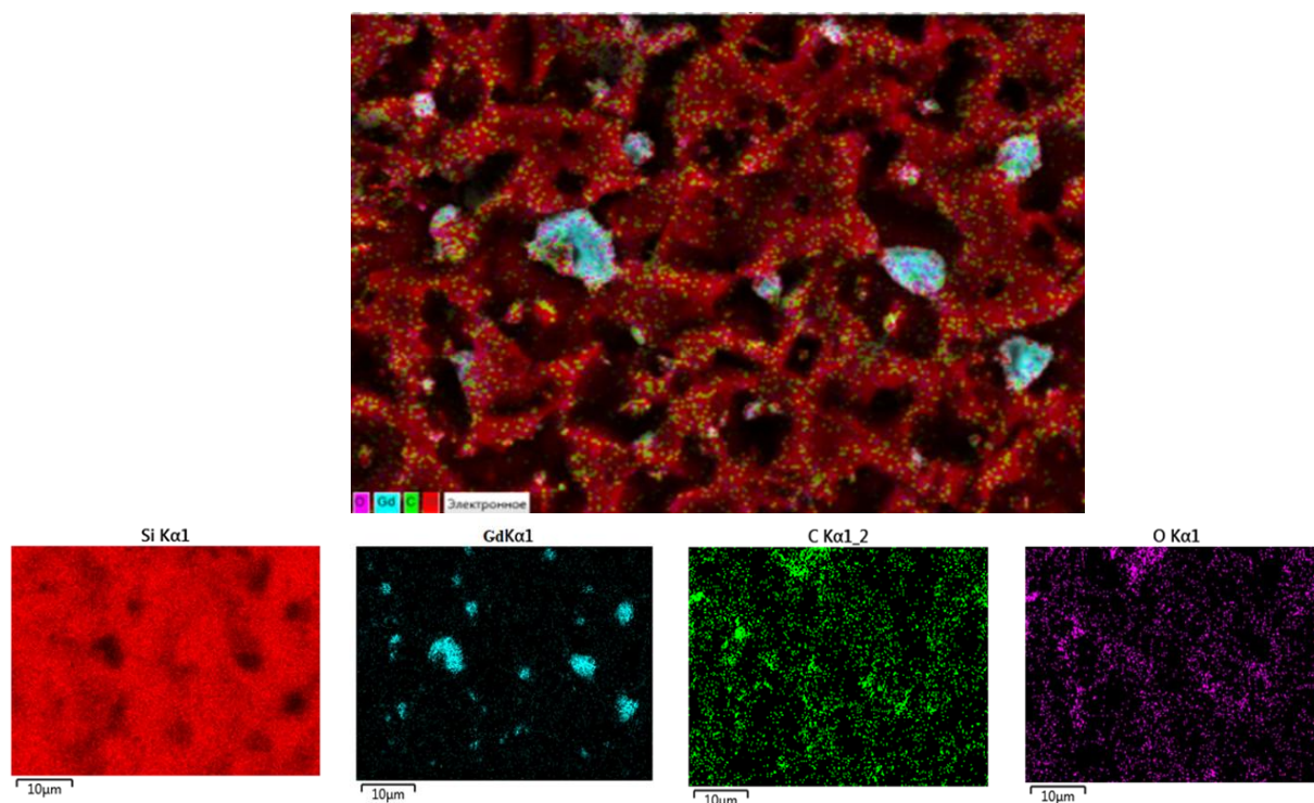
Fig.1. Energy dispersive analysis of the silicon surface sample (Si <P, Gd> - 80) doped with Gadolinium input atoms studied on the LEO-1430 SEM device.
