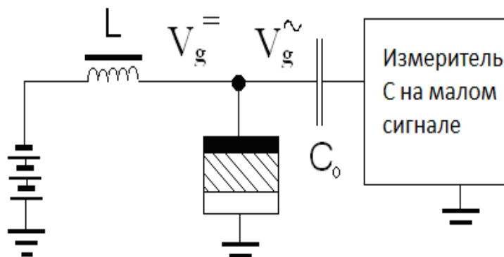
Figure 1. Schematic diagram of the measurement device for studying C–V characteristics
