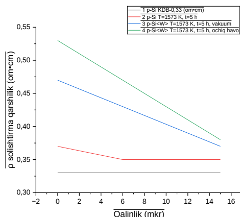
1-rasm. 1 p-Si KDB-0,33 (ohm·cm), 2 p-Si T=1573 K, t=5 h, 3 p-Si<W> T=1573 K, t=5 h, vakum, 4 p-Si<W> T=1573 K, t=5 h, ochiq havo
