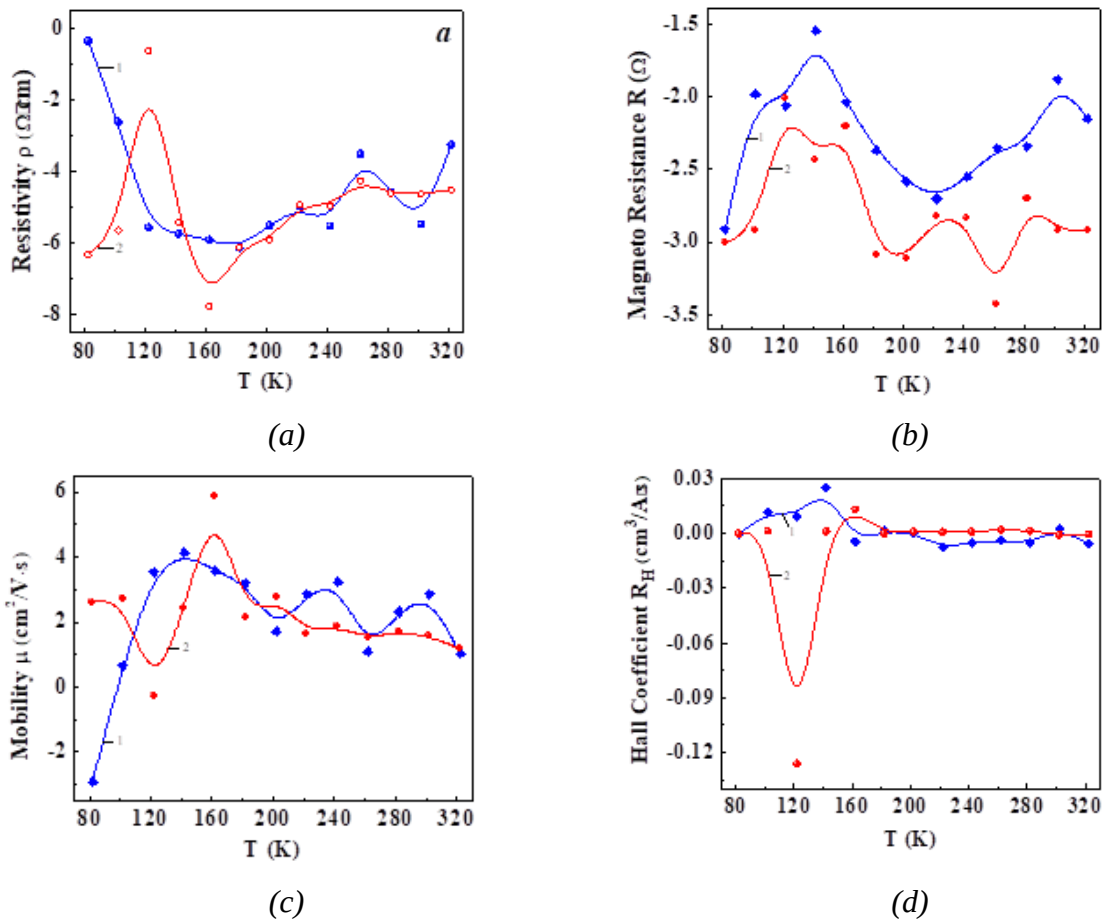
Figure 1. Temperature dependencies of resistivity (a), magnetoresistance (b), charge carrier mobility(c) and Hall coefficient(d): (1) pristine sample and (2) after 5 MeV electron irradiation to 5 \times 10^{14} \text{ cm}^{-2} at 165 K.
