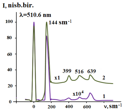
2-rasm. Oddiy (silindrsimon) kyuveta (1) va rezonatorli kyuveta (2) dagi \text{TiO}_2 mikrokukunlarining ( d_{\text{ort}}=5 \text{ mkm} ) Raman spektrlari ( I_{\text{uyg}} \sim 10^5 \text{ Vt/sm}^2 ).
