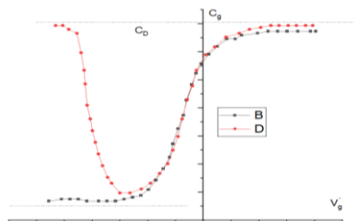
Figure 1. In MDS structures, the high-frequency and low-frequency (dashed) capacitances depend on the applied bias voltage
