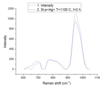
Figure 3d. Magnified view of the spectral region from 600 cm -1 to 1150 cm -1 .
