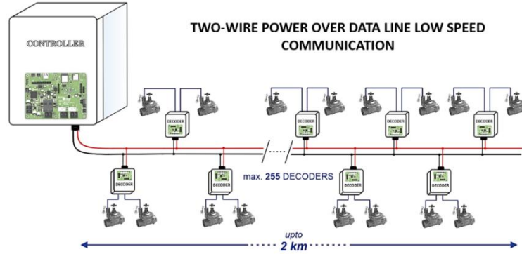
Figure 1. General structure of two-wire power over data line full-duplex
